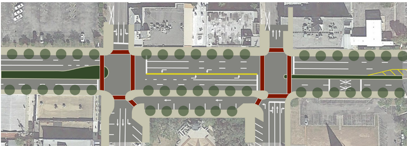
Figure 6.1: Silver Springs Boulevard and NE 1st Avenue Left Turn Diagram
